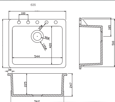
> CHEF DROP IN SINK 45L
