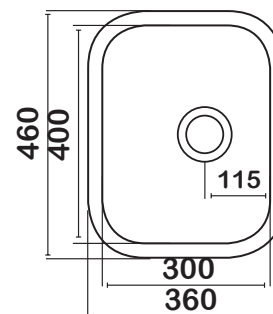
> CORAL 30 DROP IN SINK 19L Internal depth 160mm
