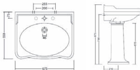
> MCKINLEY 70 CERAMIC WASH BASIN One or three tap holes
