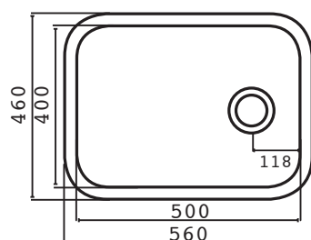
> CORAL 50 DROP IN SINK 36L Internal depth 180mm
