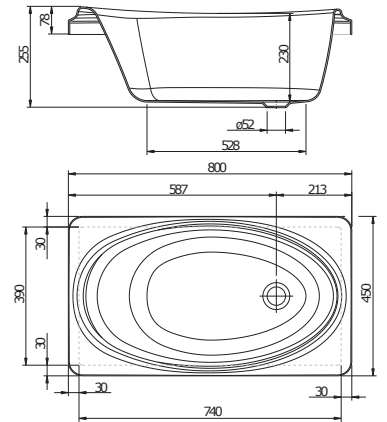
› BABY BATH 80 X 45 Acrylic
