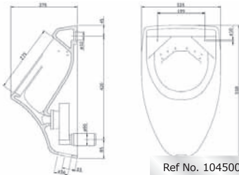
› JADE CERAMIC URINAL WITH COVER Pending approval
