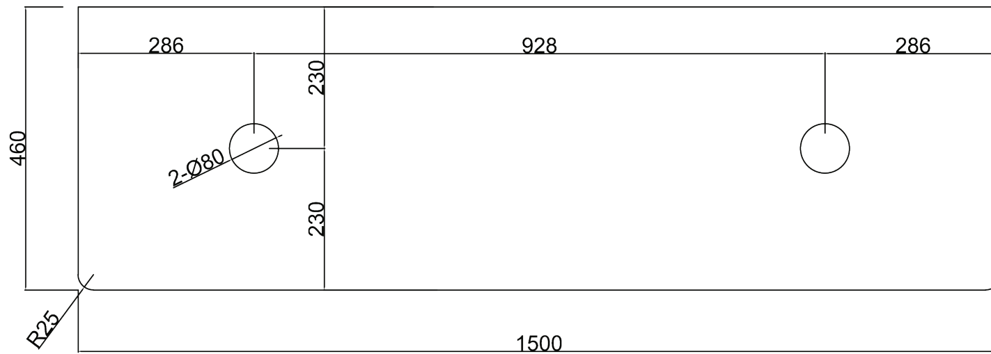
TOP VIEW W/ QUARTZ
