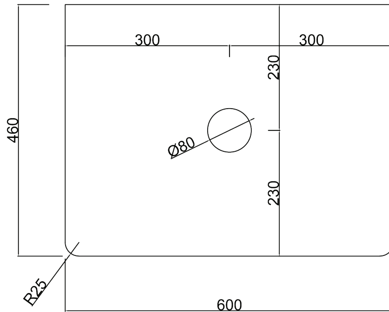
TOP VIEW W/ QUARTZ
