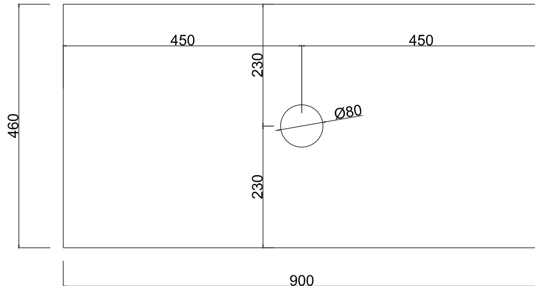
TOP W/ QUARTZ
