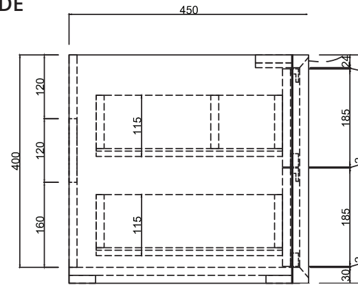
SIDE
