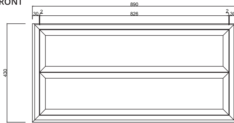
FRONT
